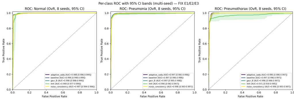
Figure 3: Class-specific error and discrimination. (a) Row-normalized confusion matrices aggregated descriptively over seeds; every row is normalized by its true class. (b) Per-class receiver-operating-characteristic curves with descriptive multi-seed 95% bands. Significant DeLong results for LMH, the noise-sensitivity (anti-consistency) condition and exploratory GACR-B reflect lower seed-42 Pneumothorax AUROC than baseline, not improvement. DeLong inference was not performed on subjects pooled across seeds.
